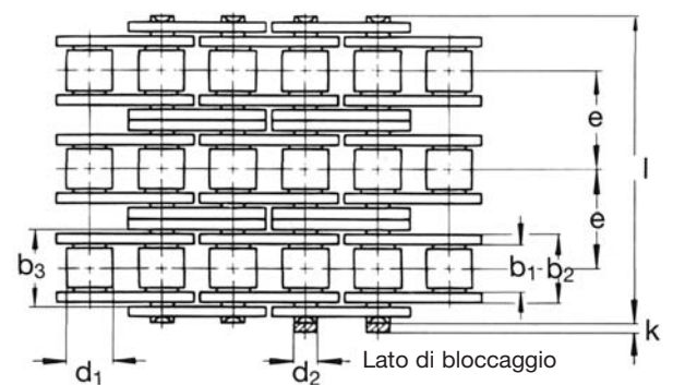
Catena a rulli tripli
